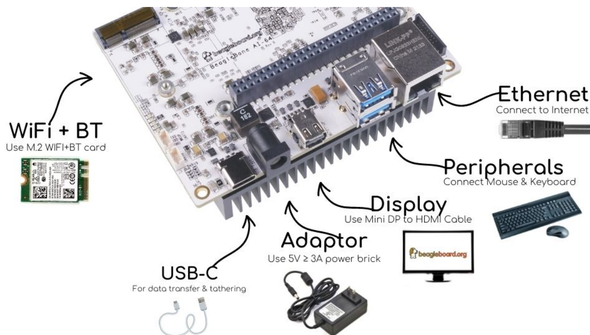
Fig. 2.8: Desktop Configuration
