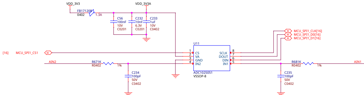
Fig. 3.6: ADC102S051 - 12bit Analog to Digital Converter (ADC)
