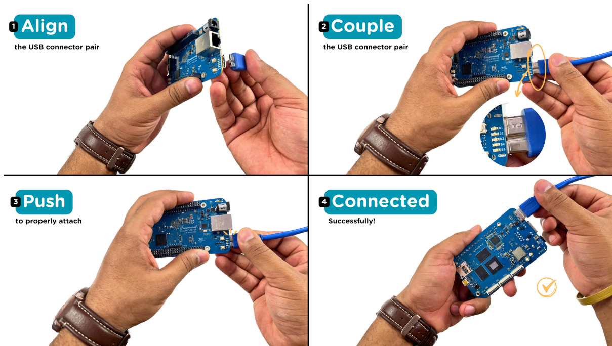
Fig. 2.4: super-speed micro-B (USB 3.0) connection guide for BeagleV-Ahead.
