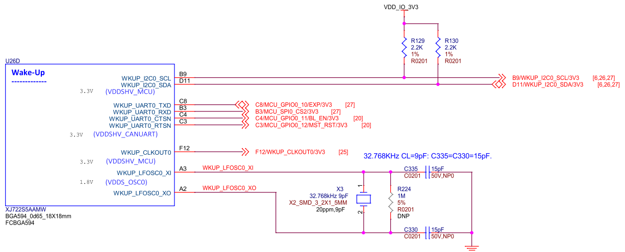
Fig. 3.6: BeagleY-AI wkup reset cntrls osc
