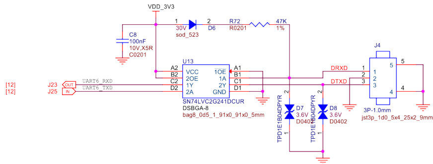
Fig. 3.42: Serial debug port
