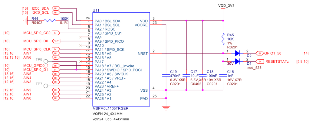
Fig. 3.41: MSPM0L1105 as 8ch 12bit ADC & 4KB EEPROM
